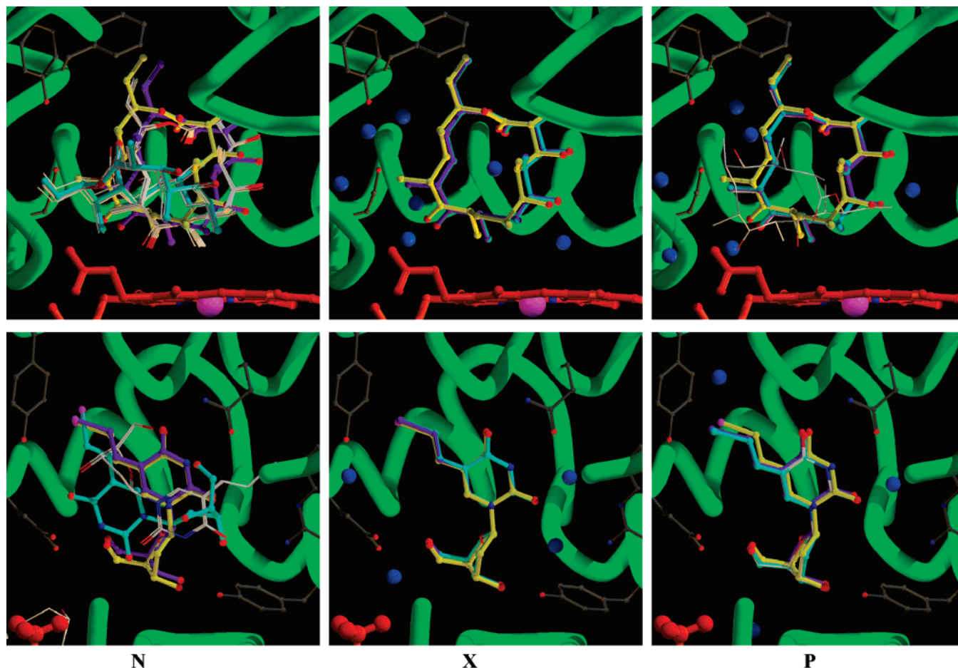
Figure 3. The effect of water and rescoring on docking accuracy. The role of water in predicting binding modes of 6-deoxyerythrulose B in the binding pocket of Cyt P450 EryF (1jio) (top) and 5-bromovinyldeoxyuridine in HSV1 TK (1ki8) (bottom), using AutoDock and different water scenarios (no water (N, left panel), X-ray water (X, middle panel), predicted water (P, right panel)). Orientations of docking solutions (white carbon atoms) ranked as no. 1 with the scoring function of AutoDock (cyan carbon atoms) and SCORE (purple carbon atoms) are compared with those observed in the crystal structure (yellow). Water oxygen atoms are depicted in blue. The figures were prepared using Molscript 55 and Raster3D. 56
